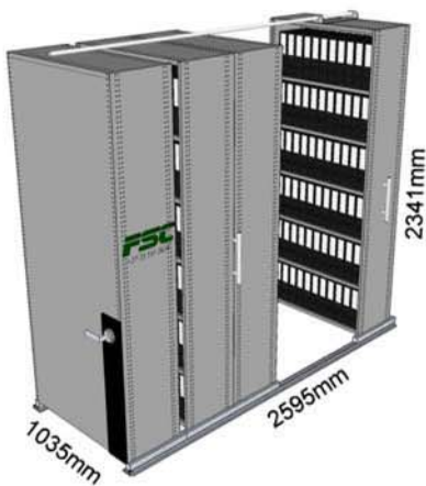
Light Duty Mobile Shelving 1 Wide 4 Bay System
